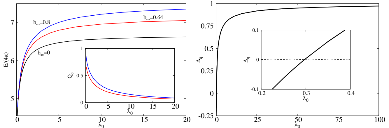
Figure 4: Left panel: The energy E and the electric charge Q_e are shown vs. the coupling constant \lambda_0 for SO(2) gauged Skyrmons in 3 + 1 dimensions, with n = 1 , \lambda_1 = \lambda_2 = \lambda_3 = 1 , and several values of b_\infty . Right panel: The relative difference \Delta_q = (q_G - q_W)/(q_G + q_W) of the individual contributions to the topological charge q = q_G + q_W = 1 is shown vs. the coupling constant \lambda_0 for the same solutions.
