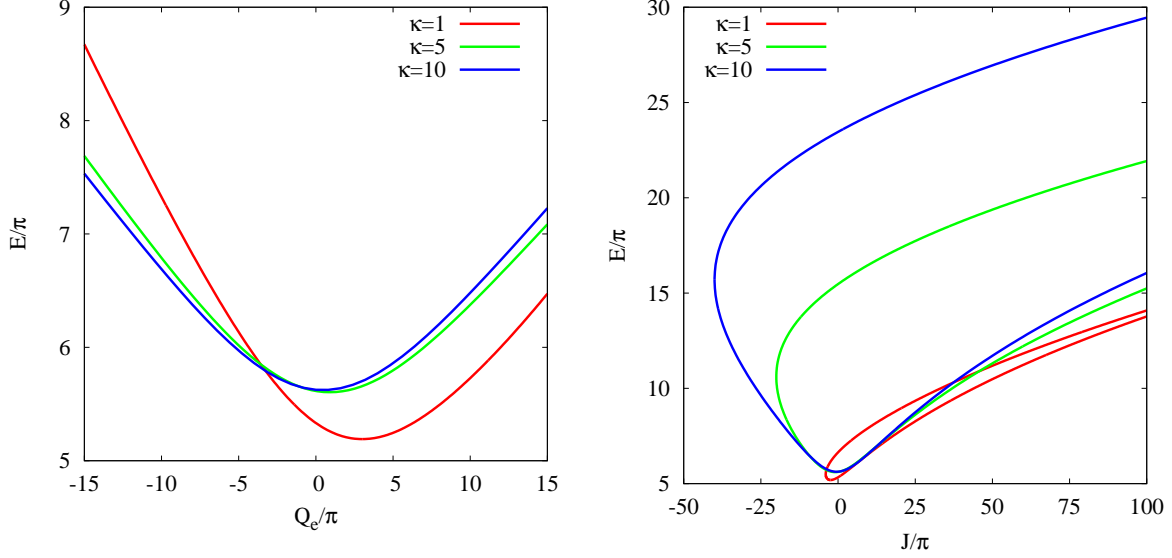
Figure 2: Left panel: Energy E vs. electric charge Q_e for vortices with n = 1 , \lambda = 1.6 , \eta = 1 , \tau = 1 , and several values of \kappa . Right panel: Energy E vs. angular momentum J for vortices with n = 1 , \lambda = 1.6 , \eta = 1 , \tau = 1 , and several values of \kappa .
