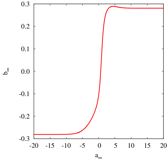
Figure 1: b_\infty vs. a_\infty for vortices with n = 1 , \lambda = 1.6 , \eta = 1 , \kappa = 1 , and \tau = 1 .
