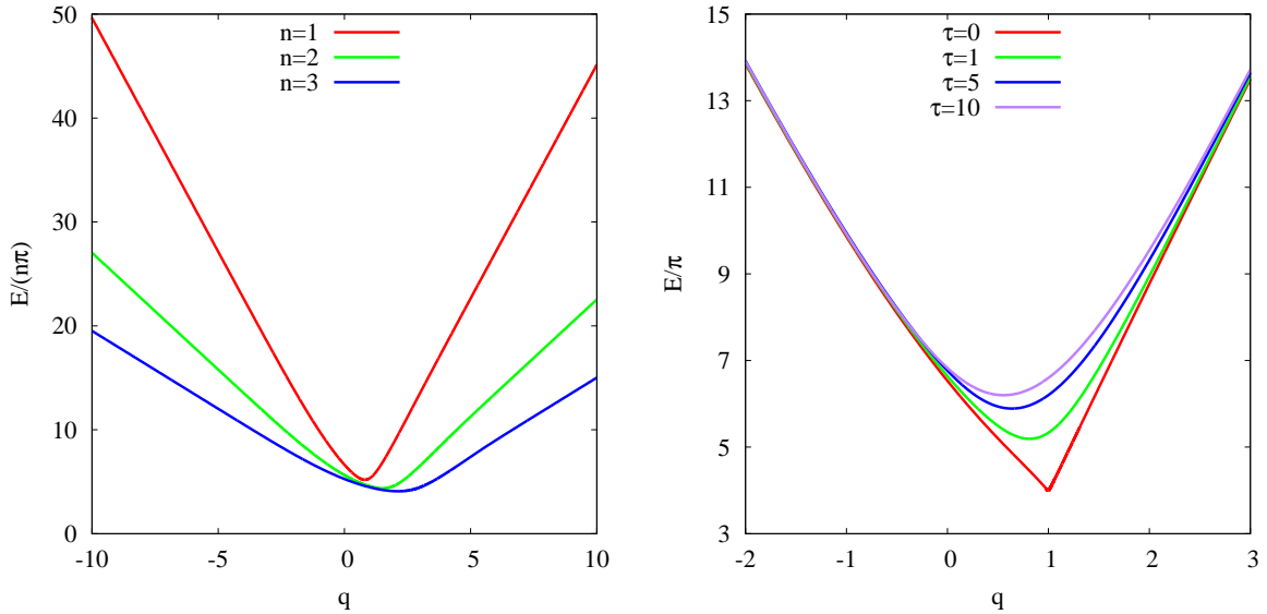
Figure 3: Left panel: Energy E vs. topological charge q for vortices with n = 1, 2, 3 , \lambda = 1.6 , \eta = 1 , \kappa = 1 , and \tau = 1 . Right panel: Same for vortices with n = 1 , \lambda = 1.6 , \eta = 1 , \kappa = 1 , and several values of \tau .
