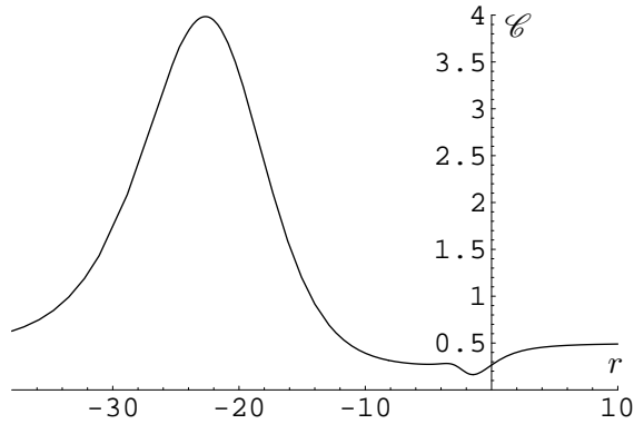
Figure 2: Cross-section through the right plot of figure 1 at g = 50 .
