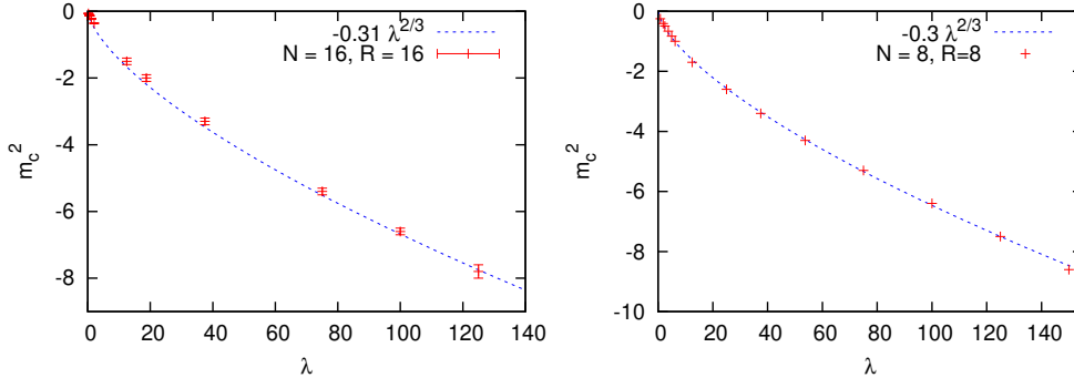
Figure 13: The phase transition at strong coupling \lambda for N = 16 , R = 16 (on the left), and for N = 8 , R = 8 (on the right). As in Figure 11 we find agreement with the matrix chain prediction m_c^2 \propto \lambda^{2/3} . In addition, comparison to the result for N = 8 , R = 16 in Figure 11 supports the full proportionality relation (6.2).
