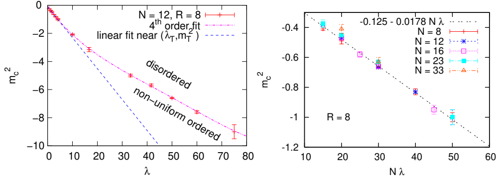
Figure 8: The transition disorder/non-uniform order at R = 8 and N = 12 (on the left), and N = 8 \dots 33 (on the right).
