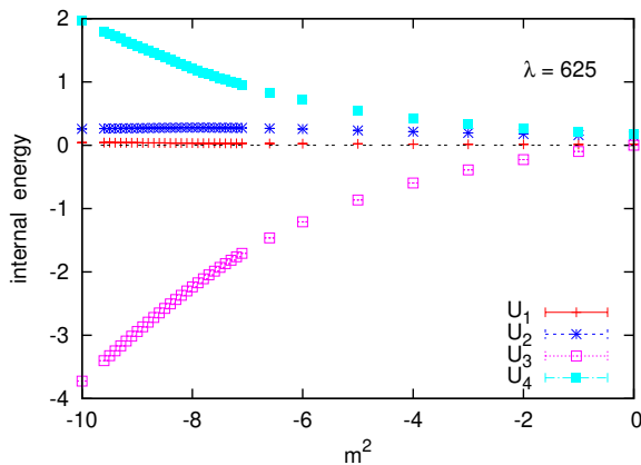
Figure 10: The different contributions to the internal energy at N = 8 , R = 16 and \lambda = 625 . The temporal kinetic contribution U_2 now clearly dominates over the spatial kinetic contribution U_1 , in contrast to the weak coupling behaviour shown in the last plot of Figure 3. This is fully consistent with the observed reduction in the spatial directions only, which leads to the matrix chain behaviour described in Ref. [26].
