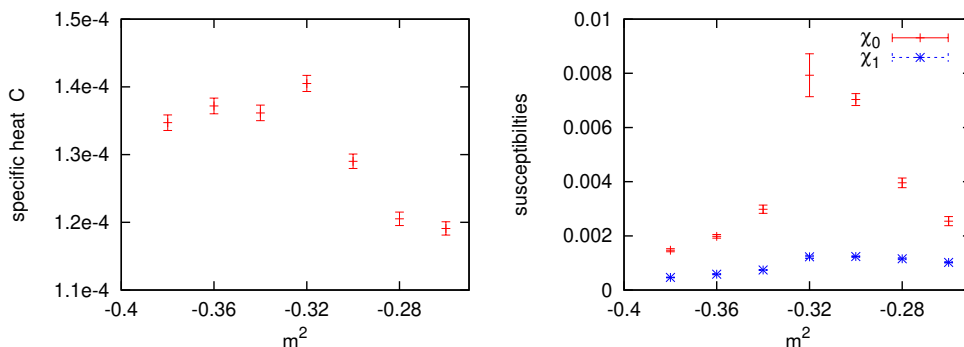
Figure 1: The specific heat C (on the left) and the susceptibilities \chi_0 and \chi_1 (on the right, defined in eq. (2.16)) for N = 16 , R = 4 and \lambda = 0.44 . The location of the maximum of C coincides with the peak in \chi_0 , which provides a consistent result for the critical value m_c^2 \simeq -0.32 .
