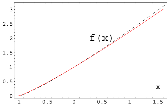
Figure 2. The scaling function f(x) for the three-dimensional XY model. The dashed line was taken from reference [15].
