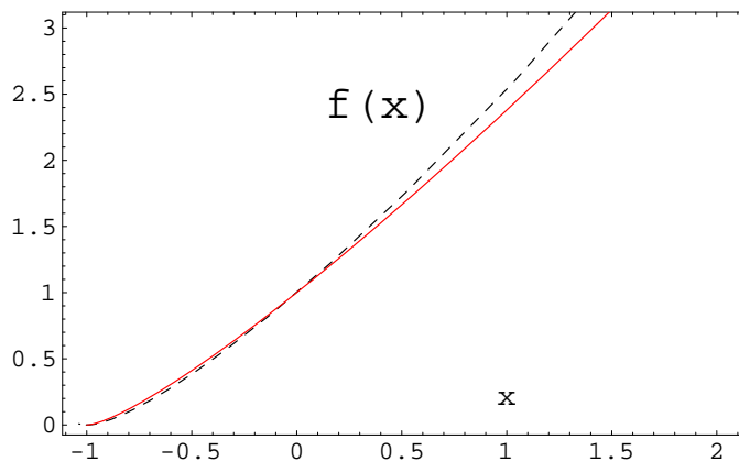
Figure 3. The scaling function f(x) for the three-dimensional Heisenberg model. The dashed line was taken from reference [13].
