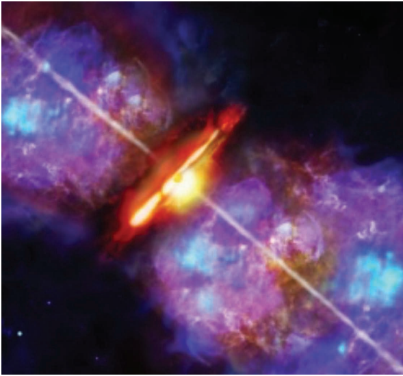
Artist's impression from Deutsches SOFIA Institute press release. Artist's impression of the accretion burst in the high-mass young star S255IR NIRS 3 (Copyright: DSI). http://www.dsi.uni-stuttgart.de/aktuelles/news/news_0056.en.html
