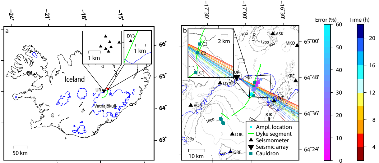
Figure 3: Projected back azimuth and amplitude location of the pre-eruptive tremor. (a) Location of UR in Iceland with respect to glaciers, the dyke (green lines) and the subaerial eruption site (red star). The insets show the geometry of UR and location of DY3 on August 30 th . (b) Amplitude location estimates of the tremor on September 3 rd 2014 are shown in the 3-4 Hz band. Lines indicate the mean back azimuth in each half hour coloured according to time. Dots indicate the best fit gridpoint in the amplitude distribution in each time window, coloured according to the minimum location error percentage. Site corrections as in supplementary table 1 were applied. Elevation in m a.s.l. based on data from the National Land Survey of Iceland. The inset shows the location of the cauldrons with respect to the back azimuth, in more detail.
