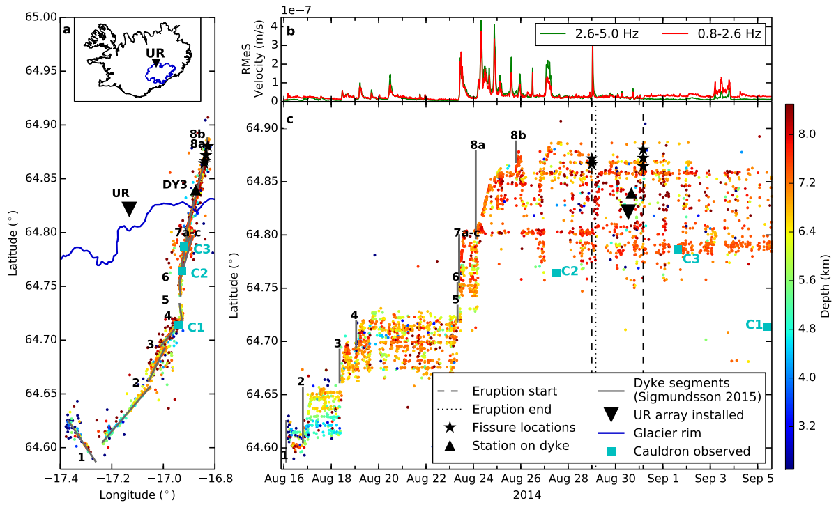
Figure 1: Earthquake locations show the propagation of the dyke at depth. (a) Dots indicate relocated earthquakes plotted in latitude and longitude from August 16 th until September 6 th , 2014 coloured according to depth (locations from figure 2c 10 ). Grey straight lines indicate dyke segments 10 . Black stars mark the location of the fissures, the black triangle the location of the temporary seismometer DY3 on top of the dyke on August 30 th and the black inverted triangle the installation of the 7-station UR seismic array. Cyan squares C1-C3 mark cauldrons and therefore potential subglacial eruption sites. The inset shows UR and Vatnajökull glacier in Iceland. (b) The Root Median Square (RMeS) of the seismic data at station KRE from the Icelandic Meteorological Office (IMO) network (see figure 3 for the location) is shown filtered between 0.8 and 2.6 and between 2.6 and 5.0 Hz. (c) Dots, grey lines, black stars, black inverted triangle and black triangle as in a. Dashed and dotted vertical lines mark the start and end of an subaerial eruption, respectively. C1-C3 mark when cauldrons were first observed during flights, or identified in aerial photos, although they might have formed earlier (pers. comm. Hannah I. Reynolds & Magnús T. Gudmundsson, Feb. 2016).
