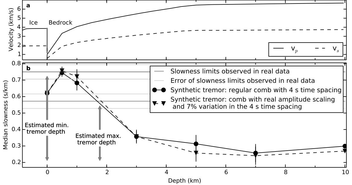
Figure 5: Tremor simulations indicate a tremor source depth of less than 2 km. (a) Velocity model for P and S waves in bedrock and ice in the volcanic zone around Vatnajökull (see Methods). (b) Median slownesses observed for synthetic tremor created with sources at different depths beneath cauldron C2. Grey horizontal lines mark the minimum and maximum slowness from array analysis of the tremor at UR array on September 3 rd , 2014. Light grey lines and black vertical lines mark the associated error in the slownesses (for details on the error estimation see section 7.1).
