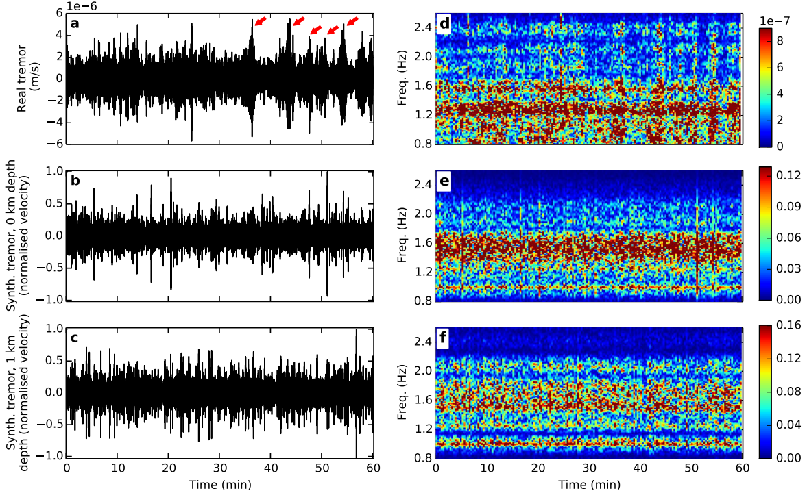
Figure 4: Comparison of real and synthetic tremor. Synthetic tremor simulated by the convolution of a simulated microseismic (Ricker wavelet) event beneath C2 recorded at UR array with a quasi-comb function with a 4 s mean time spacing, 7% time spacing variation and an amplitude distribution derived from the real tremor. (a) Horizontal velocity seismogram of real field tremor between 14:00 and 15:00 where slownesses in figure 2a indicate that the tremor source is at 1 km depth at that time, (b) Same as subfigure a but for simulated tremor from a source at 0 km depth, (c) Same as subfigure b but for a source at 1 km depth, (d) Real field tremor amplitude spectrogram, (e) Amplitude spectrogram of the simulated tremor from a source at 0 km depth and (f) Same as e but for a source at 1 km depth. All spectrograms are made with a fast Fourier transform window length of 32 s. Red arrows mark individual events in the real tremor, that are collocated with the tremor source.
