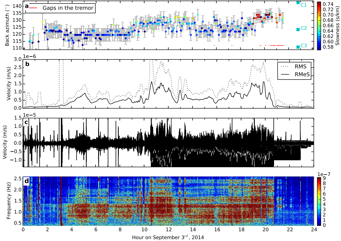
Figure 2: Laterally moving and shallowing pre-eruptive tremor on September 3 rd , 2014. (a) Dots indicate the back azimuth coloured according to horizontal slowness. The red horizontal lines indicate times when the tremor stopped completely and cyan squares mark the back azimuth of cauldrons C1-C3. (b) RMS and RMeS averaged over the vertical component of all 7 stations in UR array. (c) Instrument corrected seismogram of the vertical component at station URA of UR array filtered between 0.4 and 2.6 Hz and (d) Amplitude spectrogram of subfigure c with a fast Fourier transform window length of 256 s.
