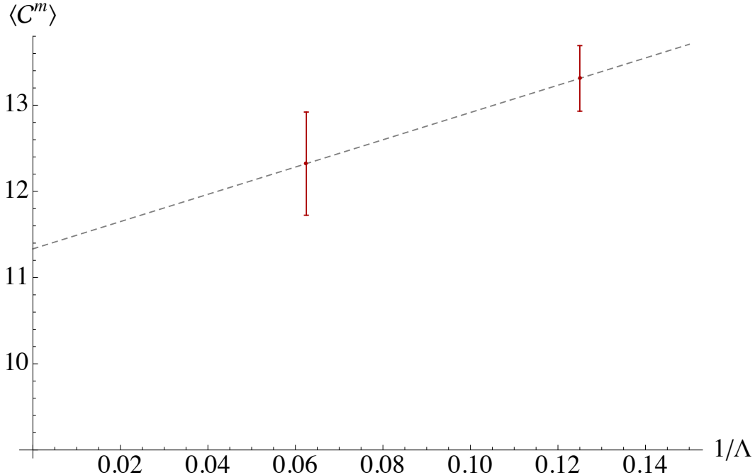
Figure 2. The red bars correspond to measurements at \Lambda = 8 and \Lambda = 16 . The extrapolated result is \langle C^m \rangle \Big|_{T=\lambda^{1/3}} = 11.33 \pm 1.26 , which is very close to the AdS/CFT prediction (3.8) for T = \lambda^{1/3} and N = 10 .
